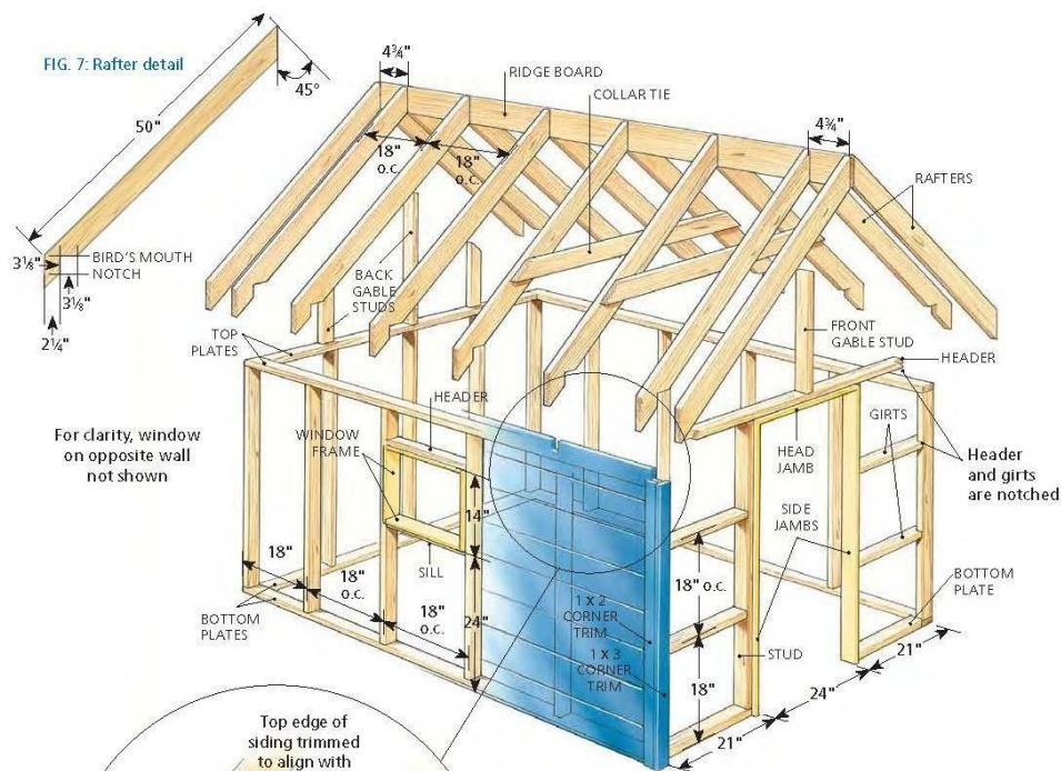
FIG. 8: Framing
